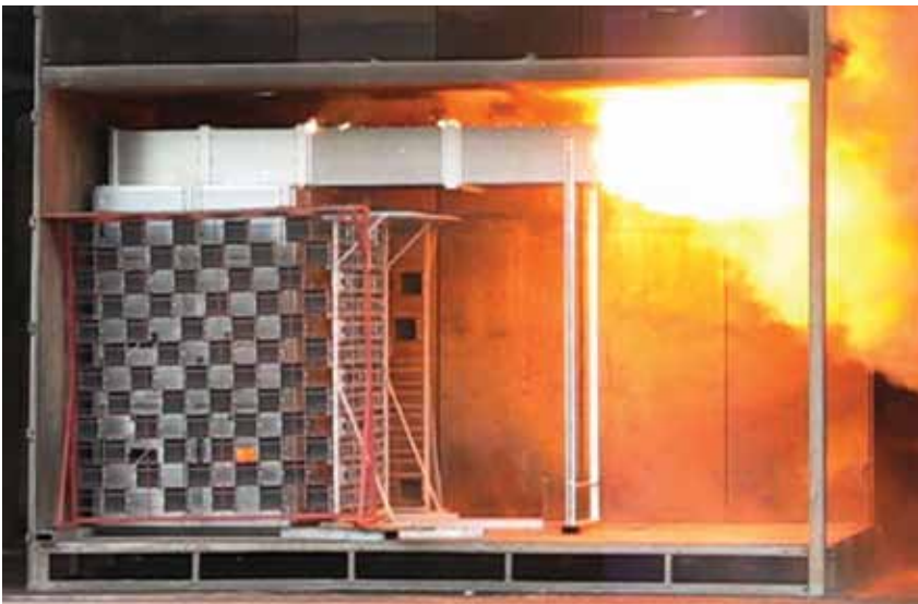
Internal arc fault test, 31.5kA/1s
